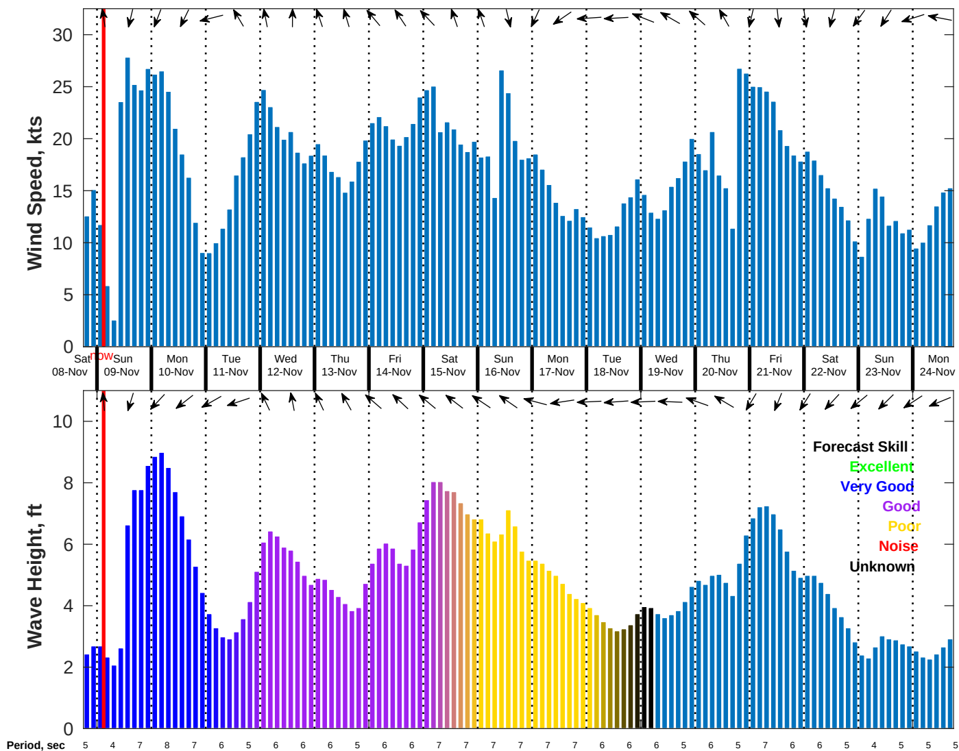
Wind & Wave Forecast for NDBC 42020 from 08-Nov-2025 18:00:00 to 24-Nov-2025 18:00:00
