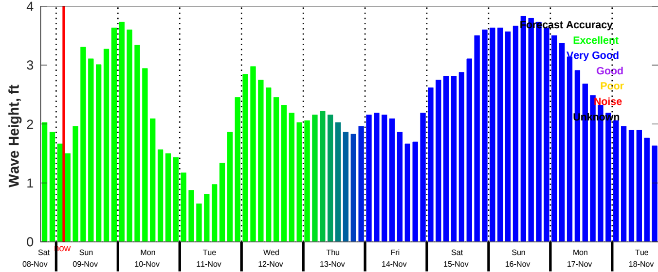
CMEMS Wave Forecast for NDBC 42035 from 08-Nov-2025 18:00:00 to 18-Nov-2025 18:00:00
