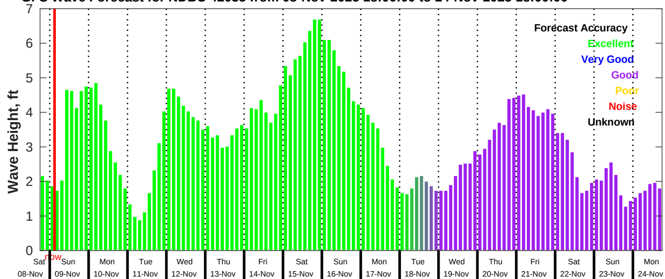
GFS Wave Forecast for NDBC 42035 from 08-Nov-2025 18:00:00 to 24-Nov-2025 18:00:00
