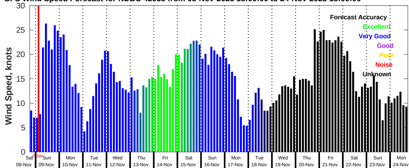
GFS Wind Speed Forecast for NDBC 42035 from 08-Nov-2025 18:00:00 to 24-Nov-2025 18:00:00
