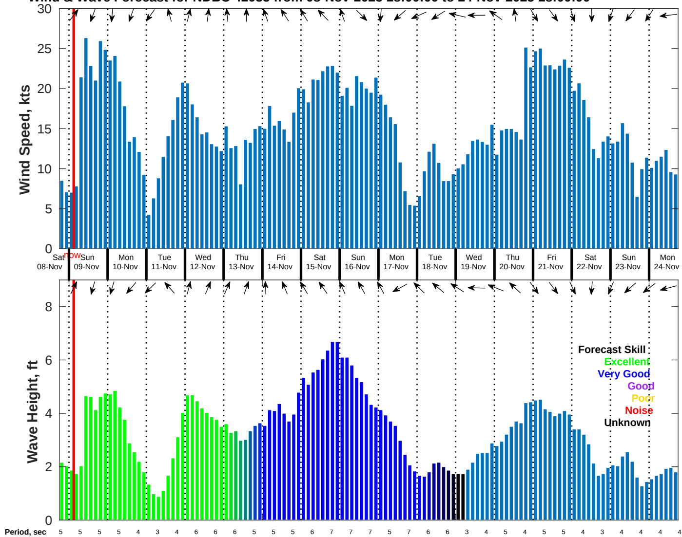
Wind & Wave Forecast for NDBC 42035 from 08-Nov-2025 18:00:00 to 24-Nov-2025 18:00:00
