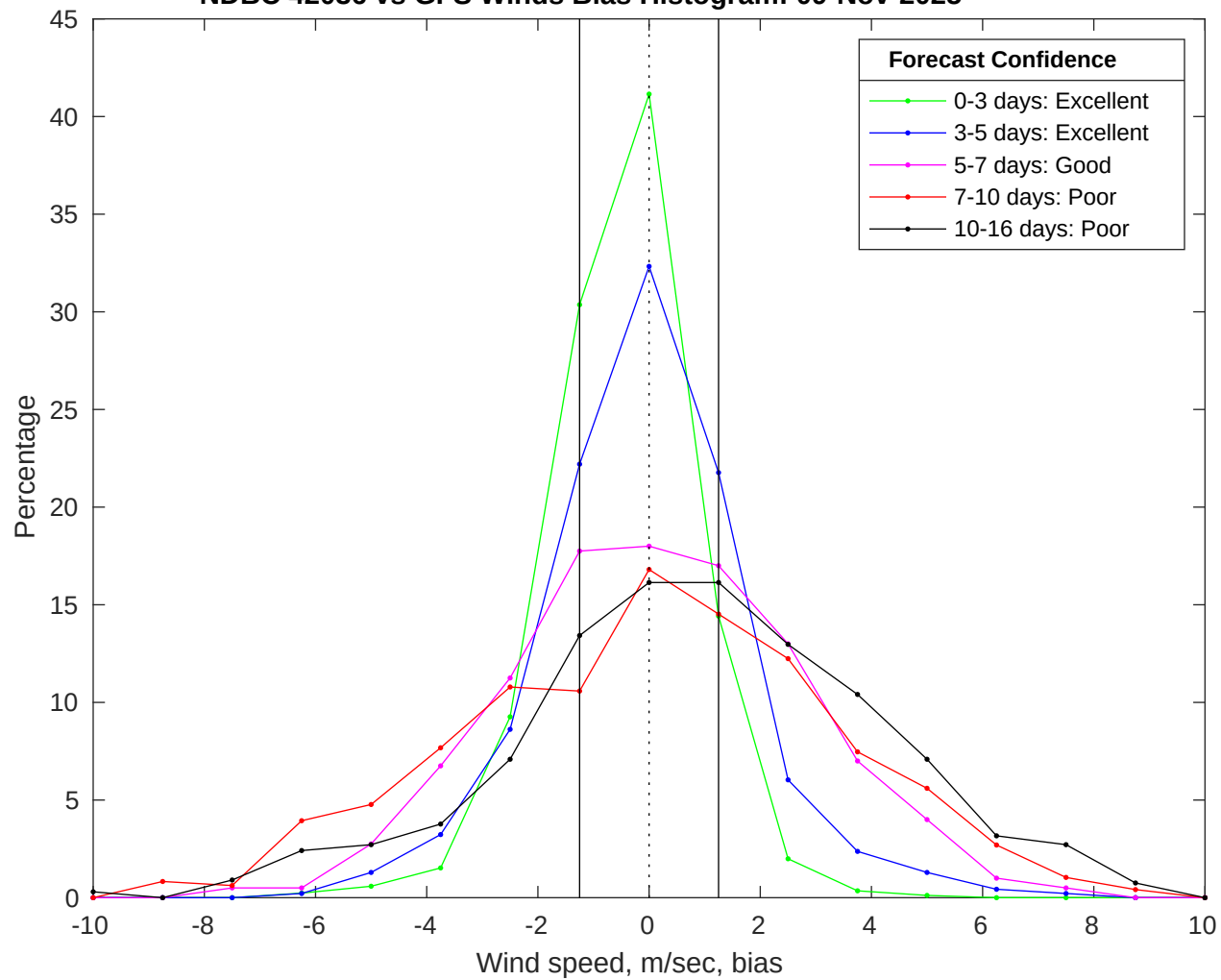
NDBC 42036 vs GFS Winds Bias Histogram: 09-Nov-2025
