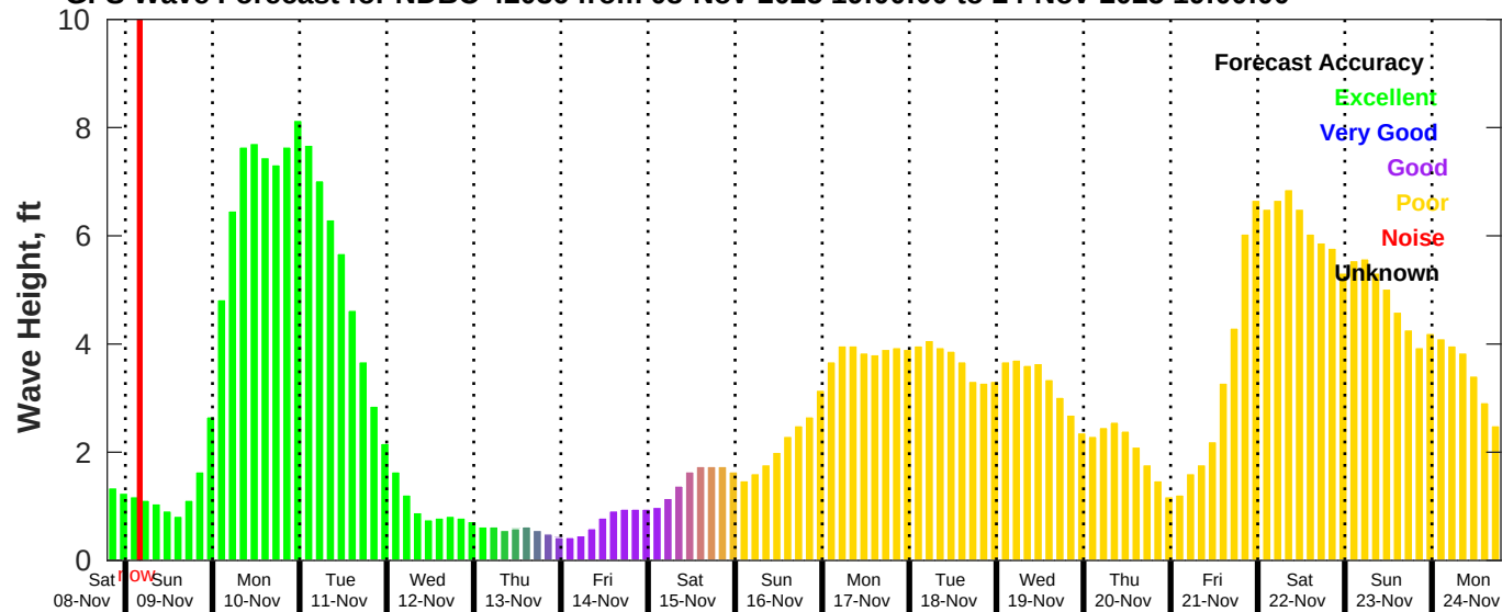
GFS Wave Forecast for NDBC 42036 from 08-Nov-2025 19:00:00 to 24-Nov-2025 19:00:00
