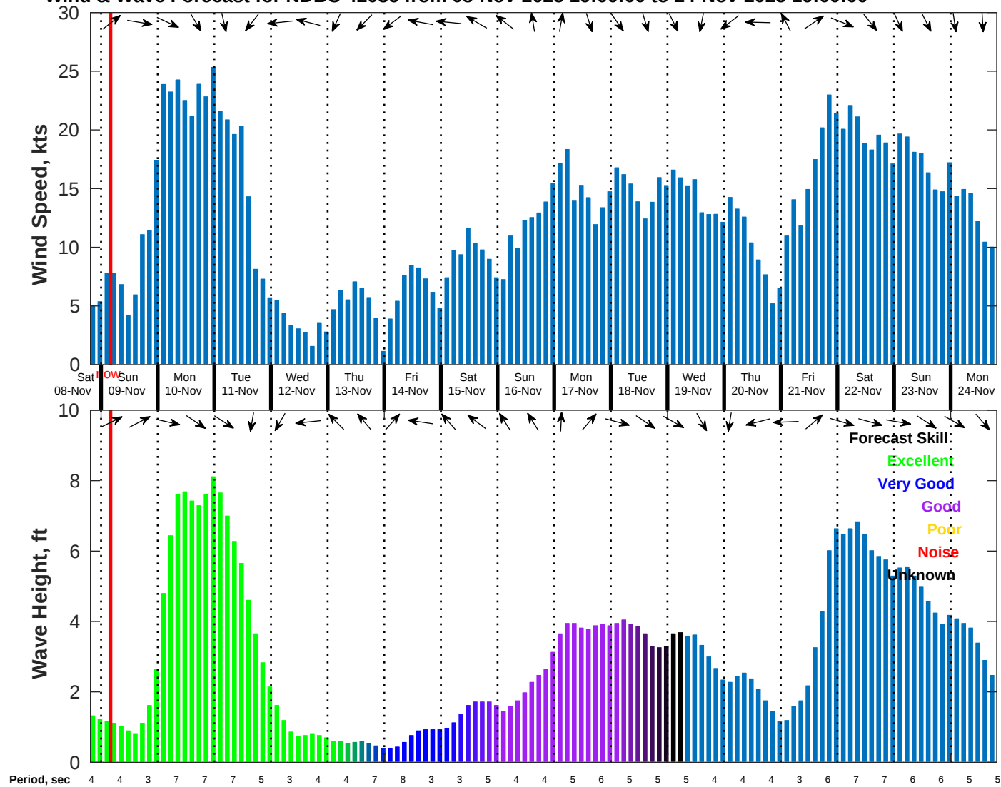
Wind & Wave Forecast for NDBC 42036 from 08-Nov-2025 19:00:00 to 24-Nov-2025 19:00:00
