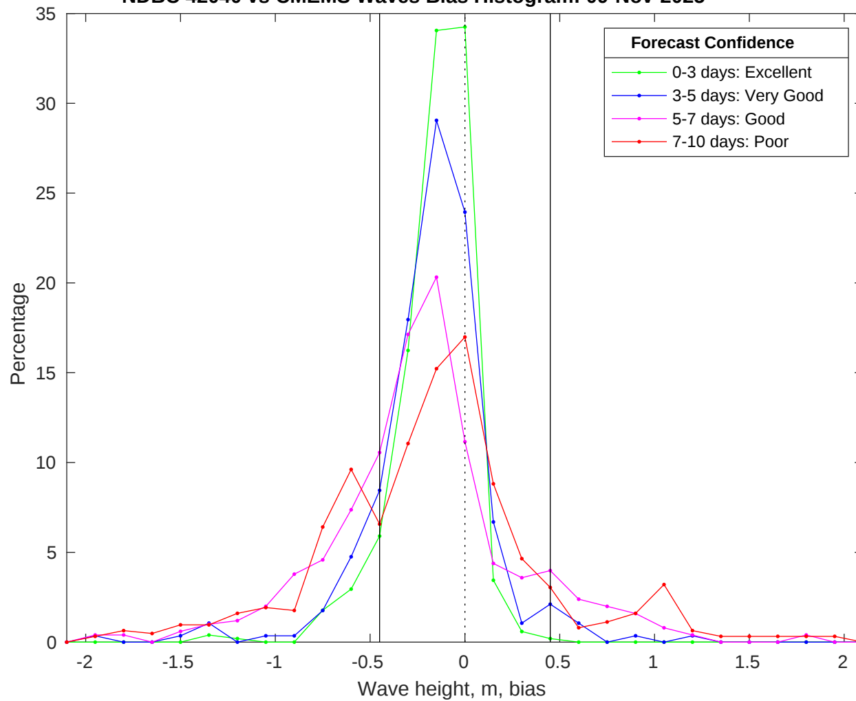
NDBC 42040 vs CMEMS Waves Bias Histogram: 09-Nov-2025
