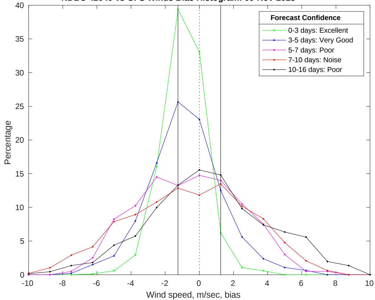
NDBC 42040 vs GFS Winds Bias Histogram: 09-Nov-2025
