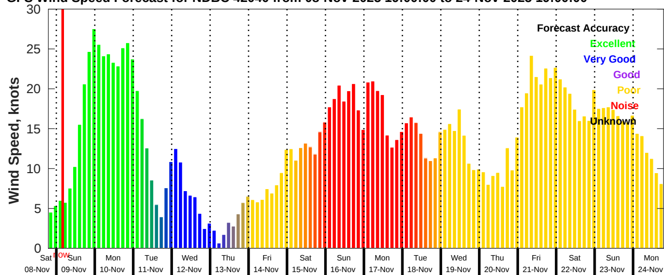
GFS Wind Speed Forecast for NDBC 42040 from 08-Nov-2025 19:00:00 to 24-Nov-2025 19:00:00
