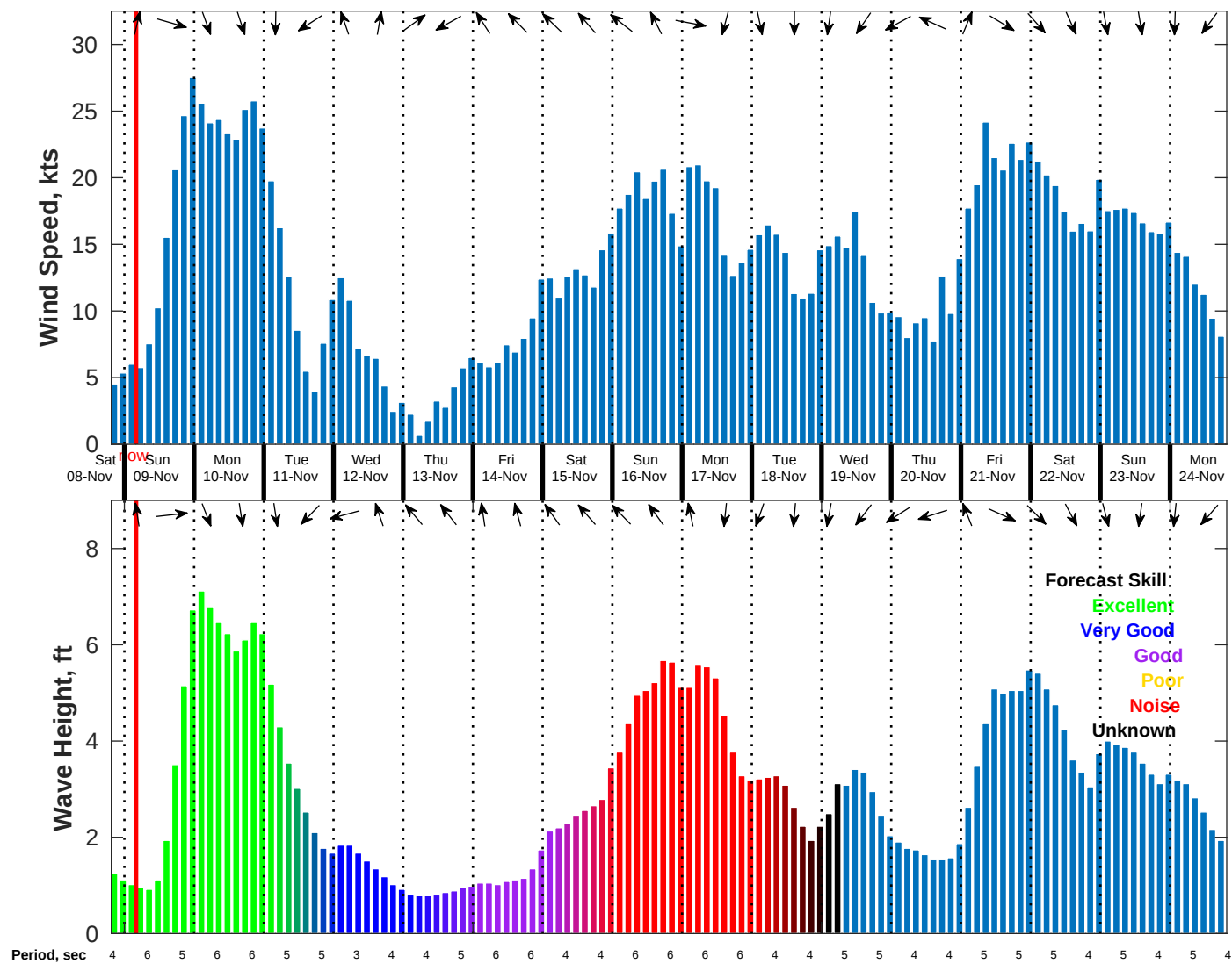
Wind & Wave Forecast for NDBC 42040 from 08-Nov-2025 19:00:00 to 24-Nov-2025 19:00:00
