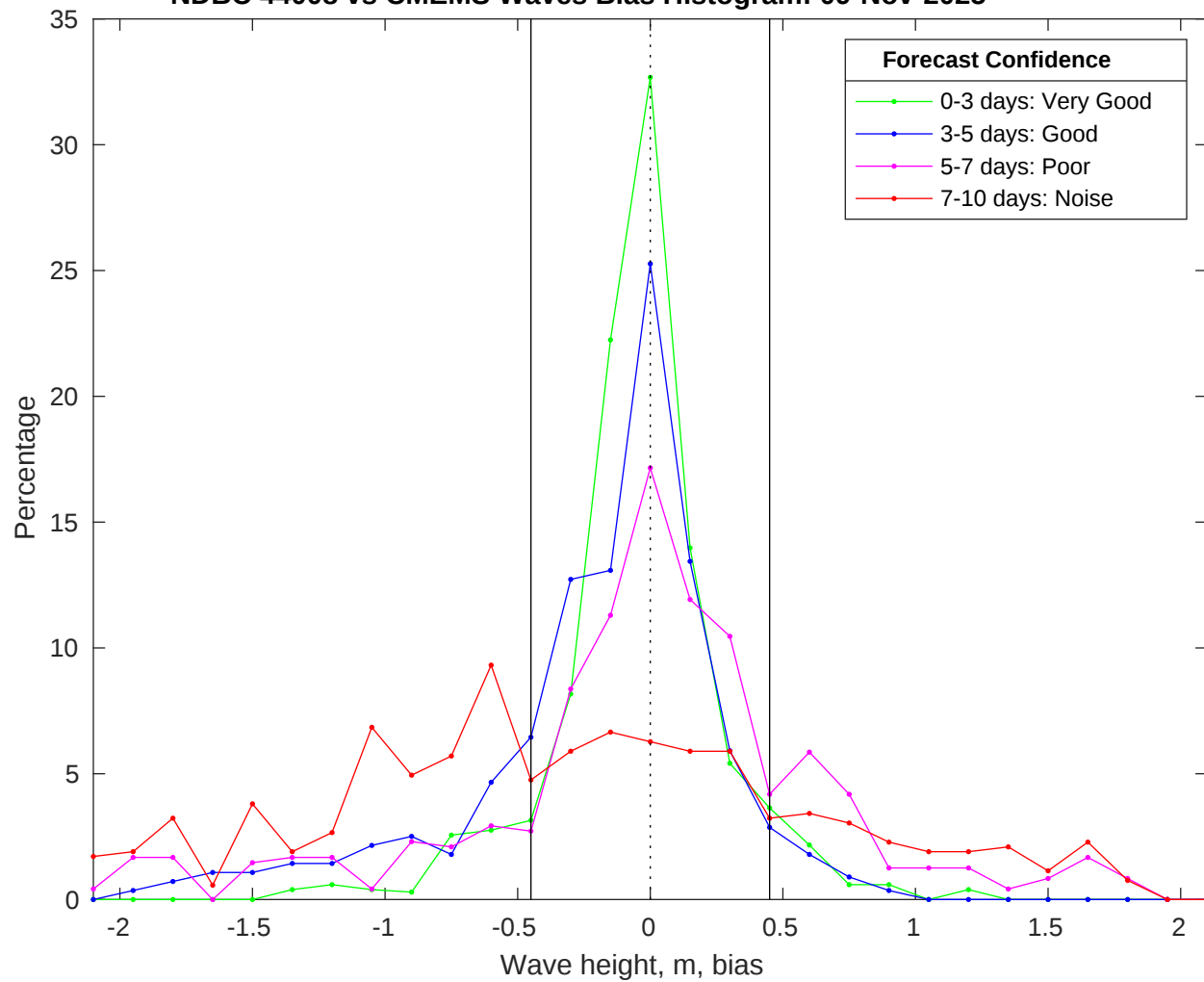
NDBC 44008 vs CMEMS Waves Bias Histogram: 09-Nov-2025
