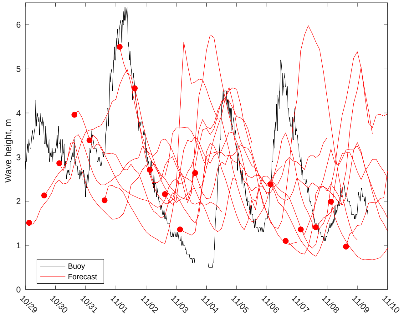
NDBC 44008 vs GFS Waves: 10 to 16 day forecast
