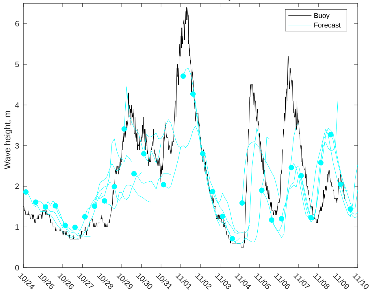
NDBC 44008 vs GFS Waves: 5 to 7 day forecast
