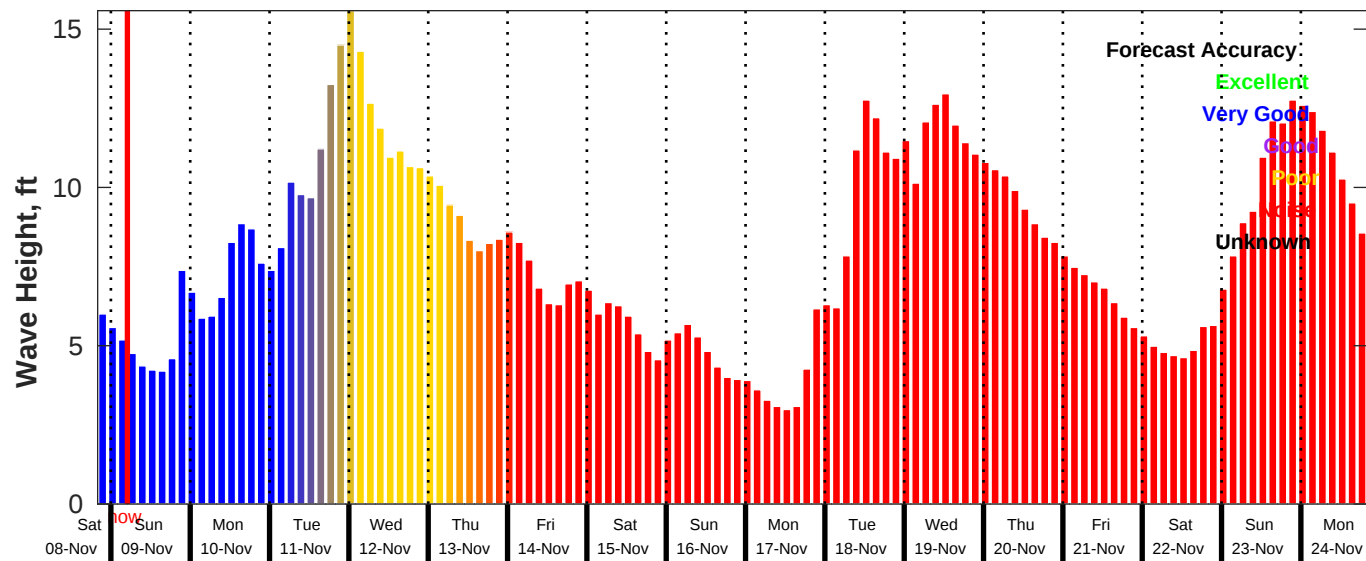
GFS Wave Forecast for NDBC 44008 from 08-Nov-2025 20:00:00 to 24-Nov-2025 20:00:00
