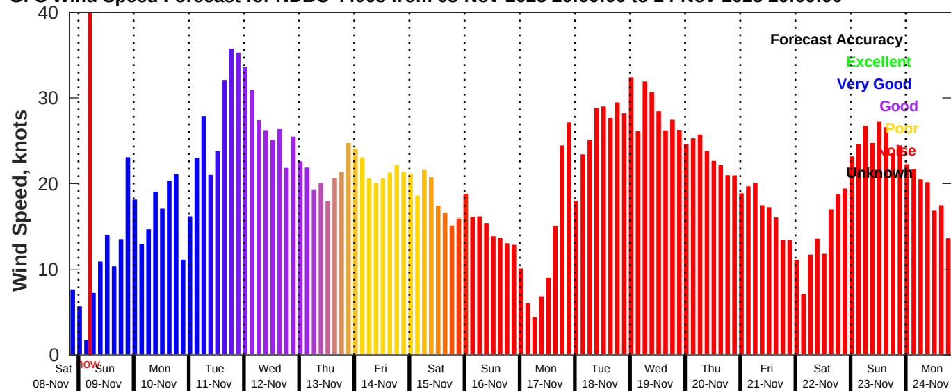
GFS Wind Speed Forecast for NDBC 44008 from 08-Nov-2025 20:00:00 to 24-Nov-2025 20:00:00
