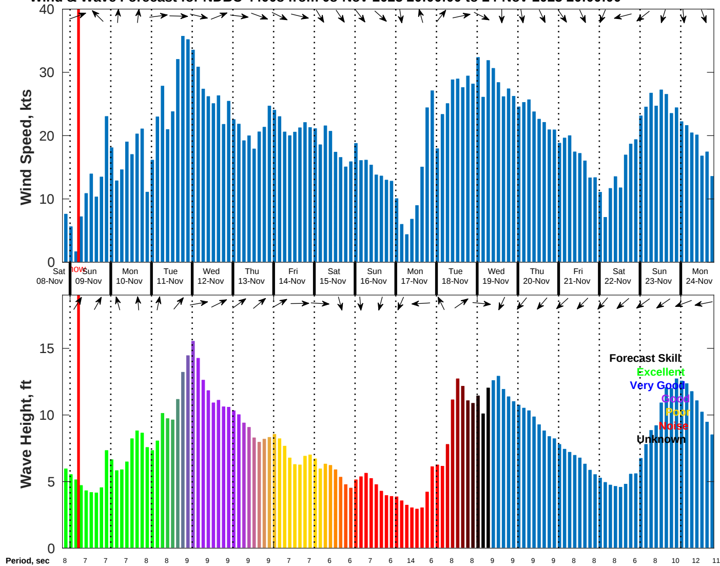
Wind & Wave Forecast for NDBC 44008 from 08-Nov-2025 20:00:00 to 24-Nov-2025 20:00:00
