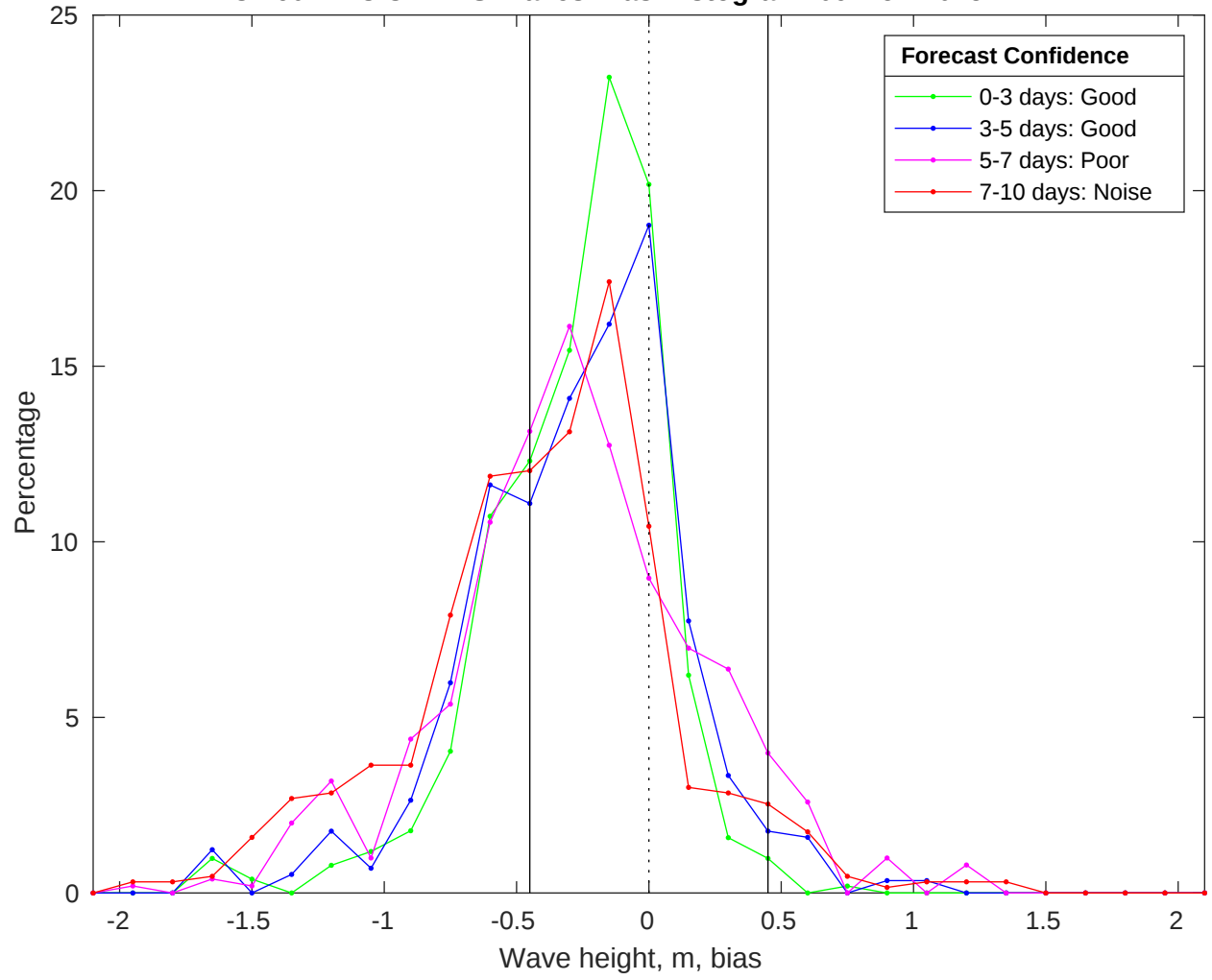
NDBC 46011 vs CMEMS Waves Bias Histogram: 09-Nov-2025
