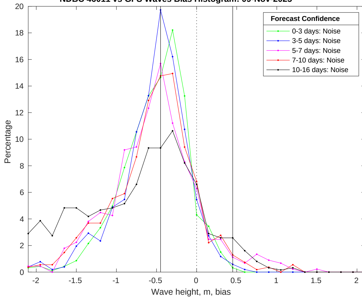
NDBC 46011 vs GFS Waves Bias Histogram: 09-Nov-2025
