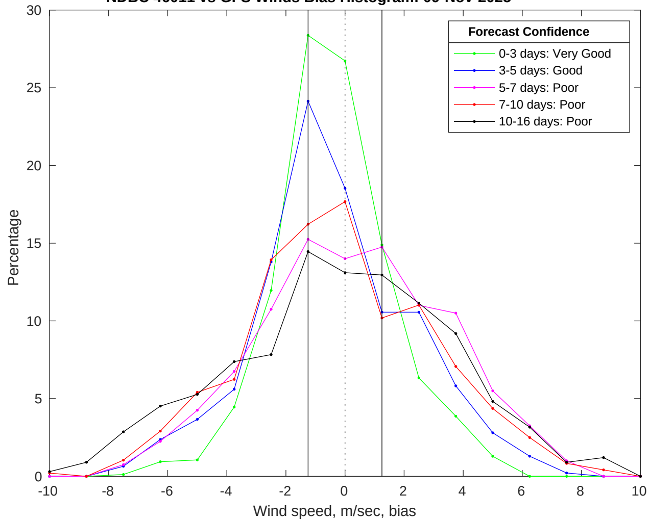
NDBC 46011 vs GFS Winds Bias Histogram: 09-Nov-2025
