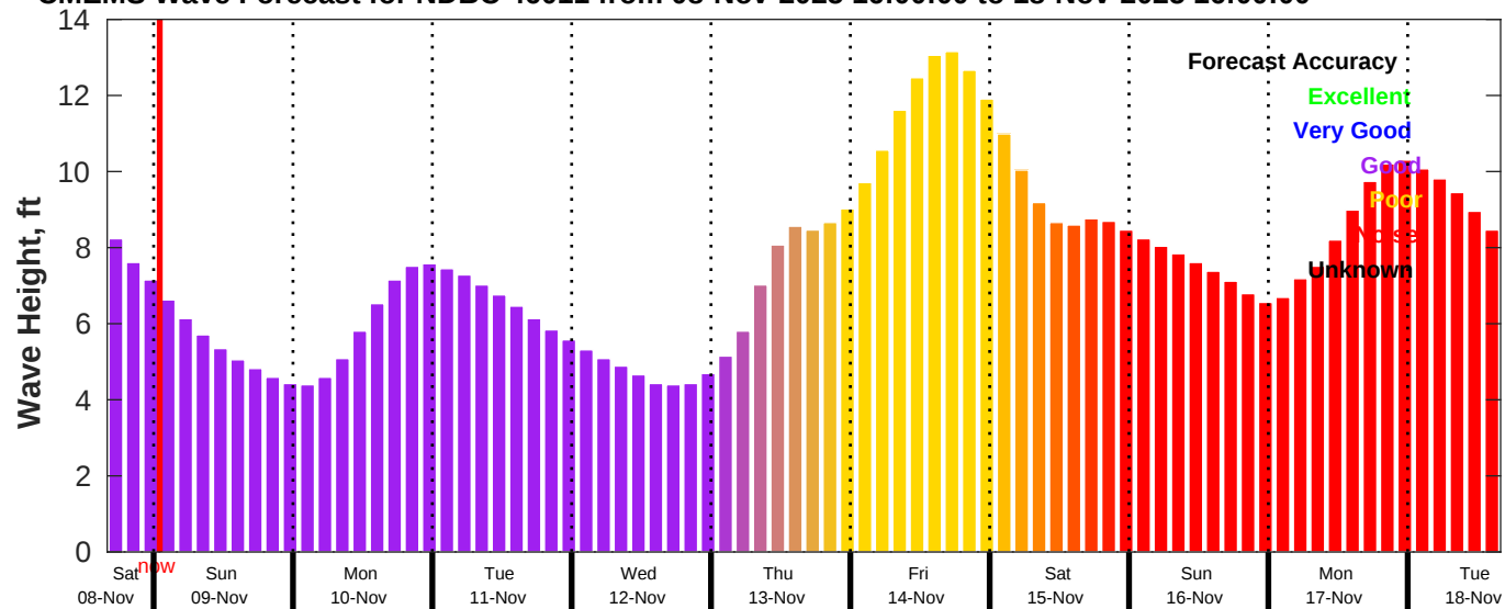
CMEMS Wave Forecast for NDBC 46011 from 08-Nov-2025 16:00:00 to 18-Nov-2025 16:00:00
