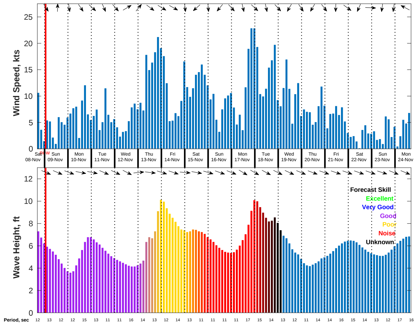
Wind & Wave Forecast for NDBC 46011 from 08-Nov-2025 16:00:00 to 24-Nov-2025 16:00:00
