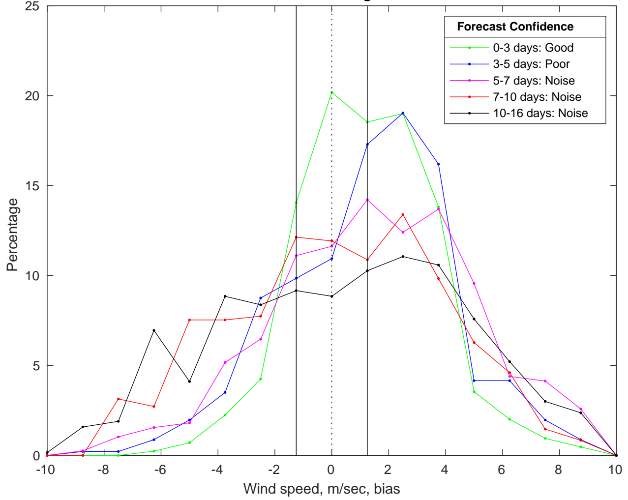
NDBC 46028 vs GFS Winds Bias Histogram: 09-Nov-2025
