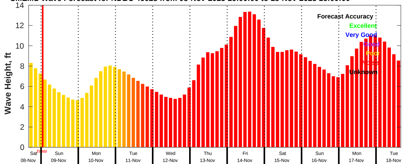
CMEMS Wave Forecast for NDBC 46028 from 08-Nov-2025 16:00:00 to 18-Nov-2025 16:00:00
