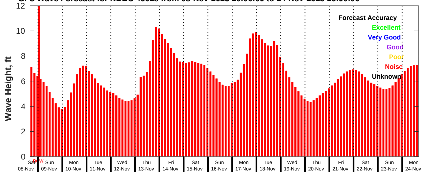
GFS Wave Forecast for NDBC 46028 from 08-Nov-2025 16:00:00 to 24-Nov-2025 16:00:00
