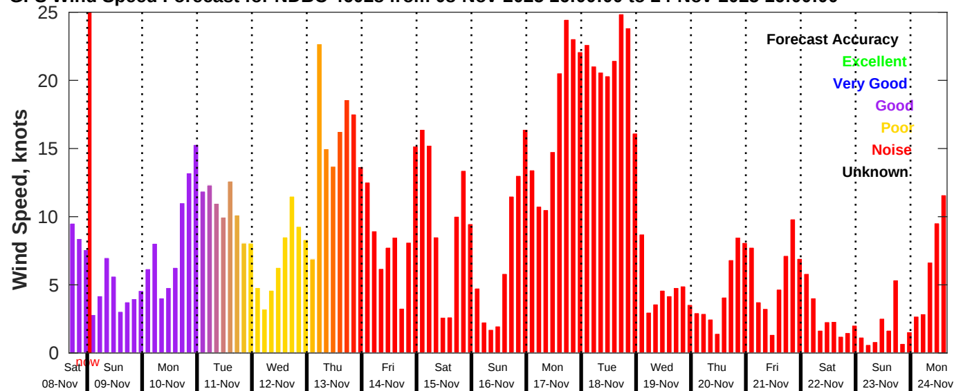
GFS Wind Speed Forecast for NDBC 46028 from 08-Nov-2025 16:00:00 to 24-Nov-2025 16:00:00
