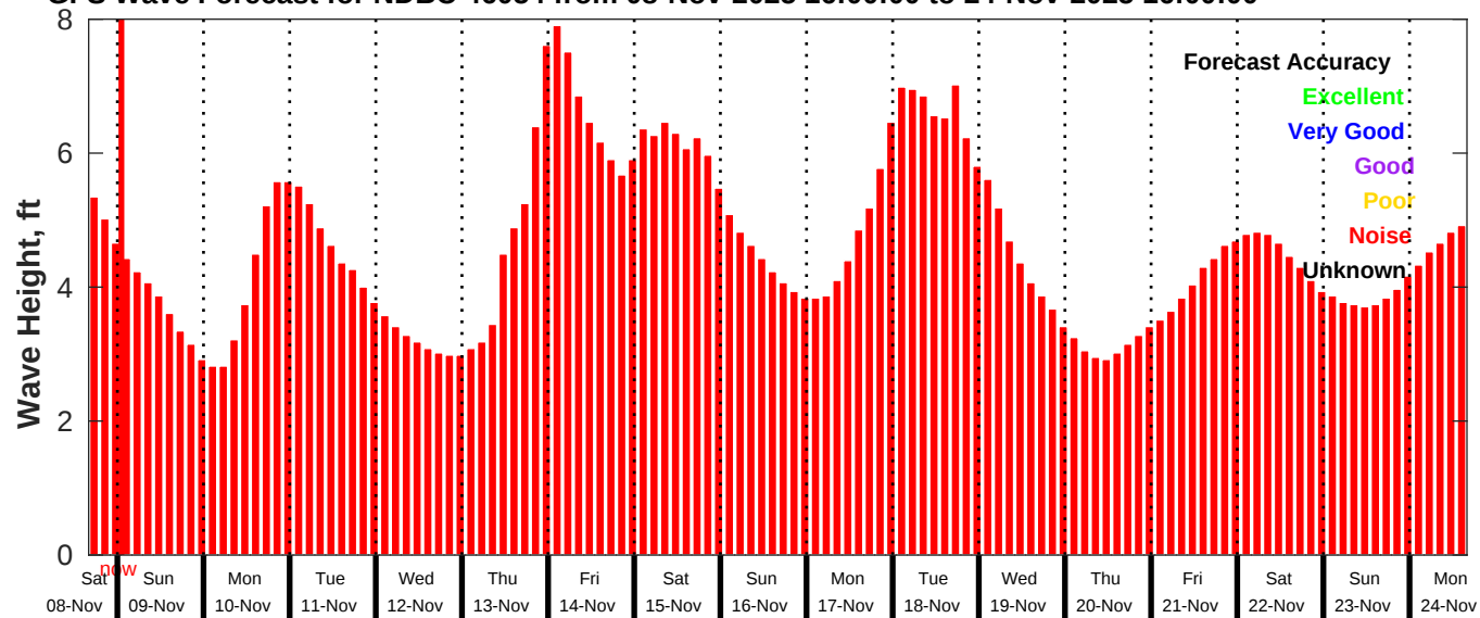
GFS Wave Forecast for NDBC 46054 from 08-Nov-2025 16:00:00 to 24-Nov-2025 16:00:00
