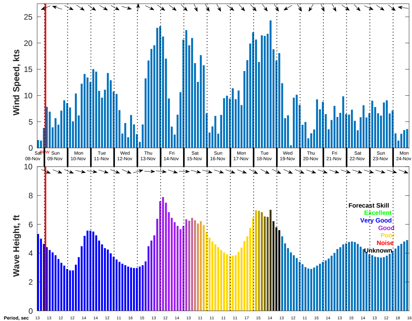
Wind & Wave Forecast for NDBC 46054 from 08-Nov-2025 16:00:00 to 24-Nov-2025 16:00:00
