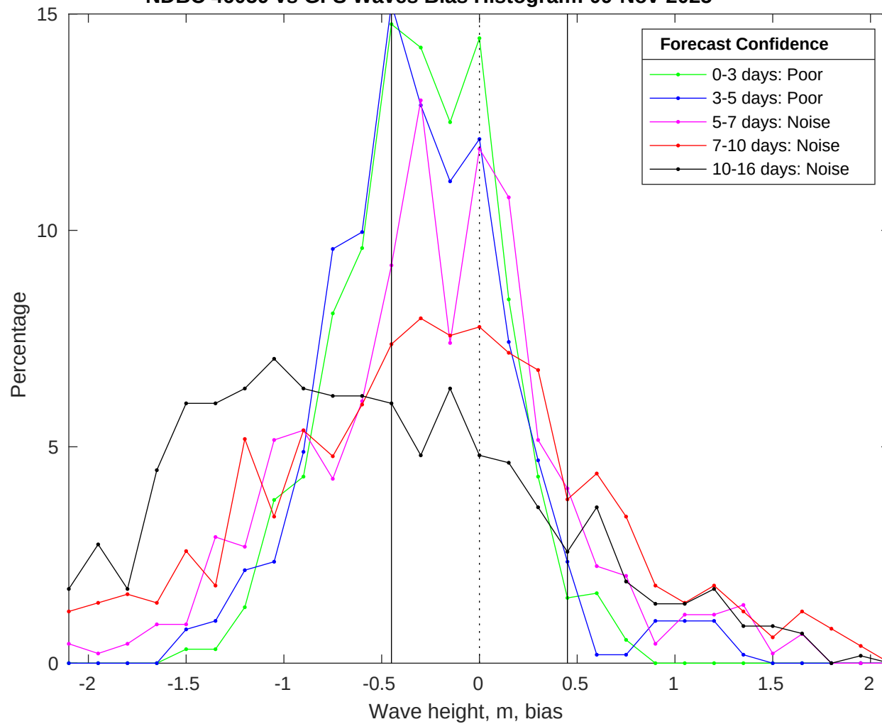
NDBC 46059 vs GFS Waves Bias Histogram: 09-Nov-2025
