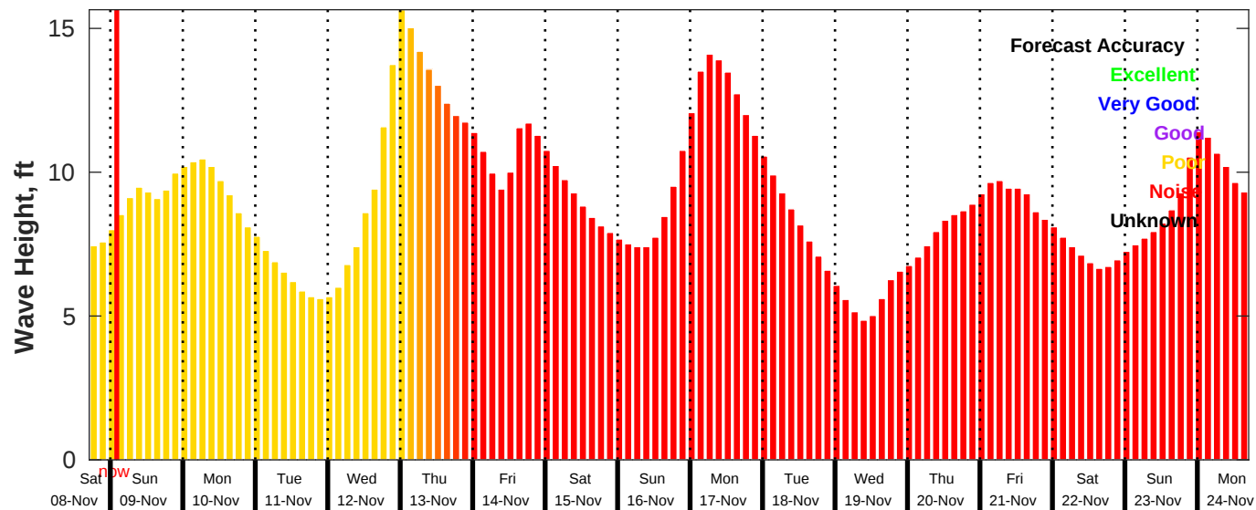
GFS Wave Forecast for NDBC 46059 from 08-Nov-2025 17:00:00 to 24-Nov-2025 17:00:00
