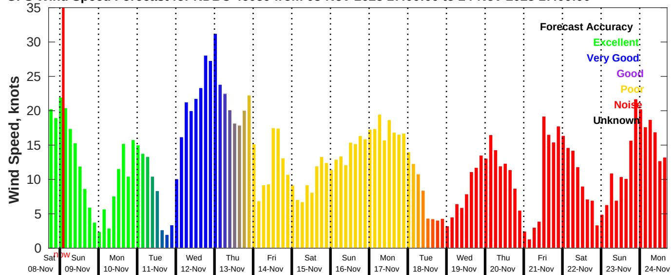
GFS Wind Speed Forecast for NDBC 46059 from 08-Nov-2025 17:00:00 to 24-Nov-2025 17:00:00
