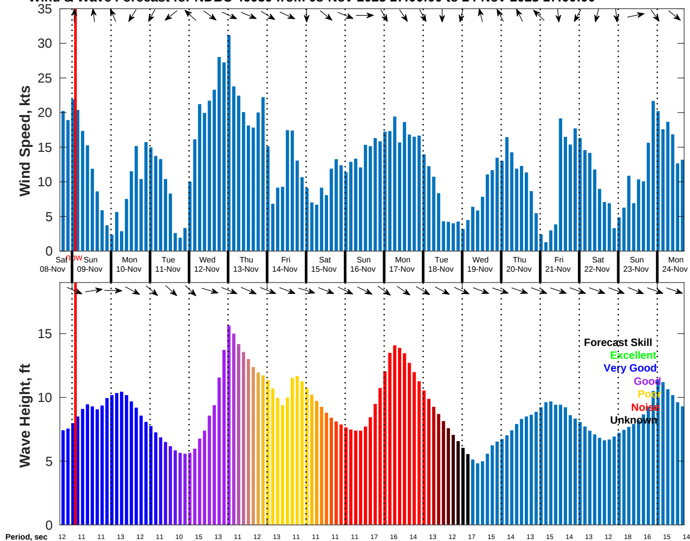
Wind & Wave Forecast for NDBC 46059 from 08-Nov-2025 17:00:00 to 24-Nov-2025 17:00:00
