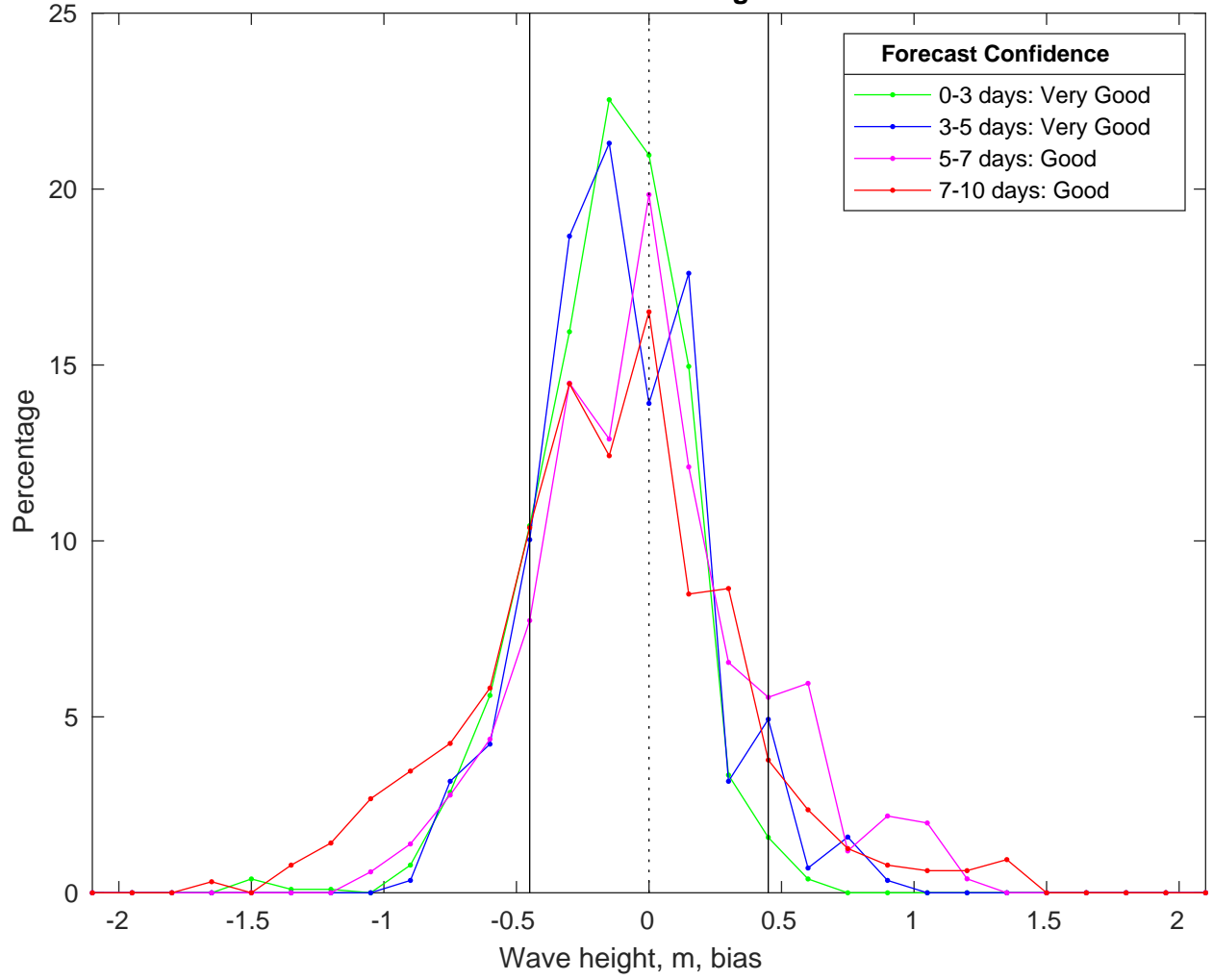
NDBC 46069 vs CMEMS Waves Bias Histogram: 09-Nov-2025
