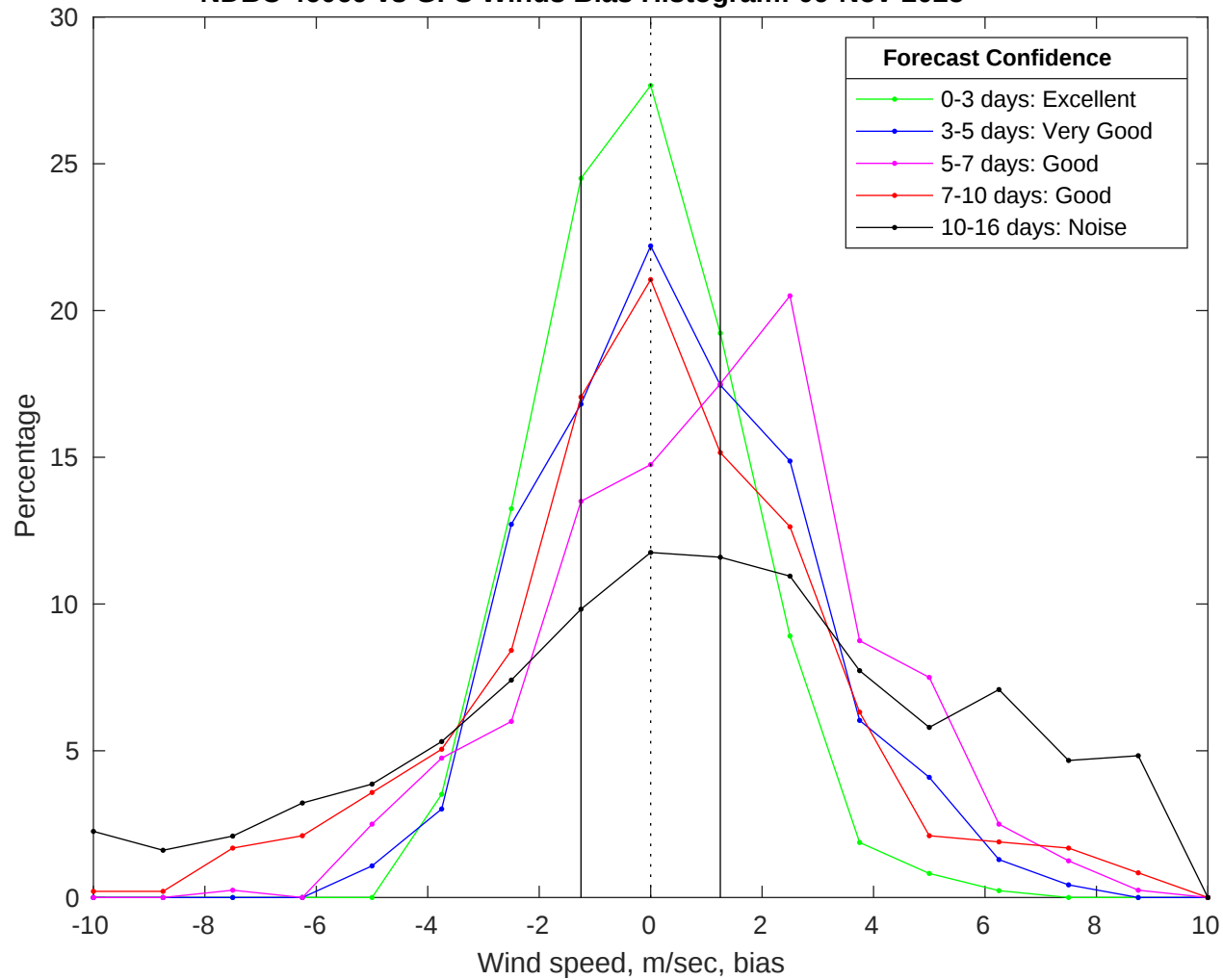
NDBC 46069 vs GFS Winds Bias Histogram: 09-Nov-2025
