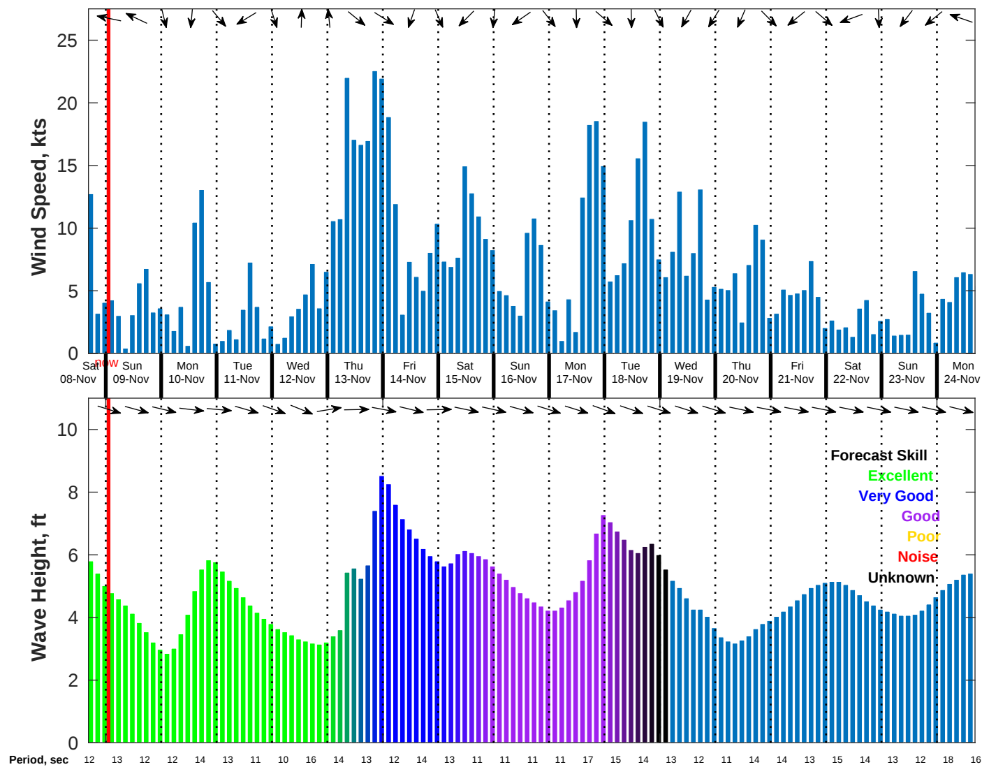
Wind & Wave Forecast for NDBC 46215 from 08-Nov-2025 16:00:00 to 24-Nov-2025 16:00:00
