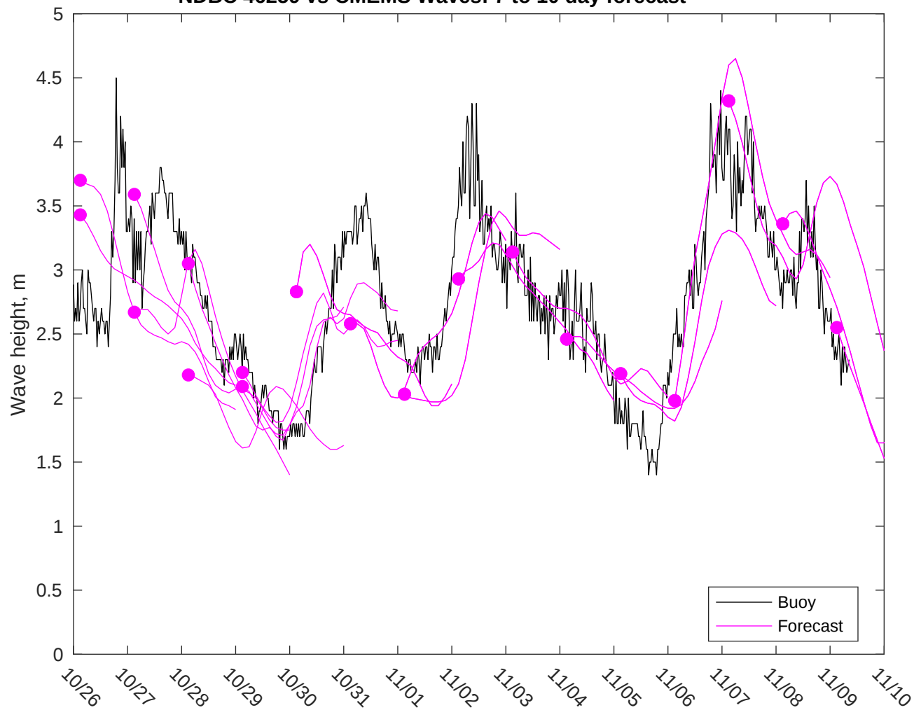
NDBC 46259 vs CMEMS Waves: 7 to 10 day forecast
