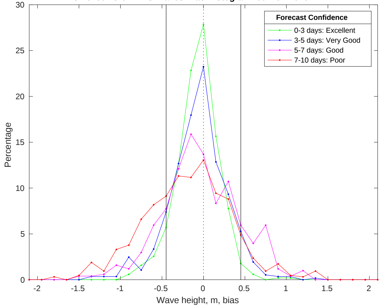
NDBC 46259 vs CMEMS Waves Bias Histogram: 09-Nov-2025
