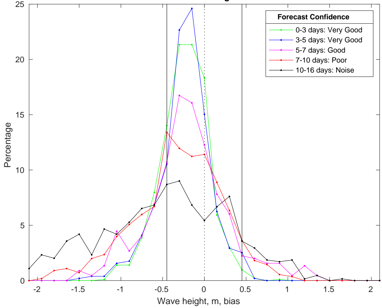
NDBC 46259 vs GFS Waves Bias Histogram: 09-Nov-2025
