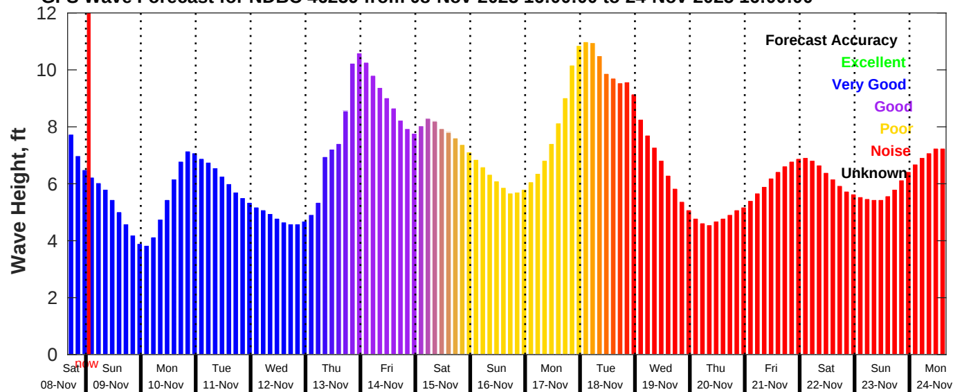
GFS Wave Forecast for NDBC 46259 from 08-Nov-2025 16:00:00 to 24-Nov-2025 16:00:00
