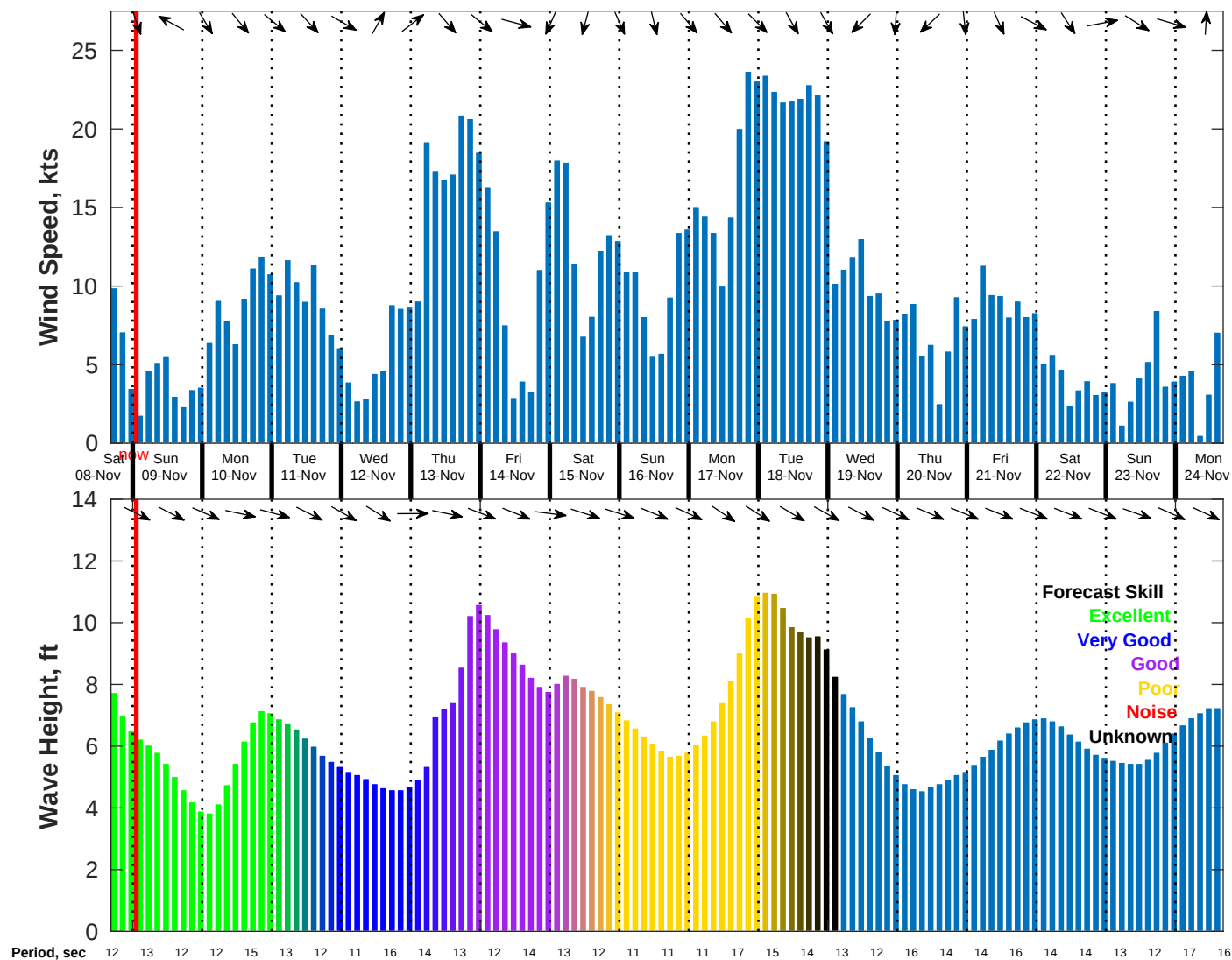
Wind & Wave Forecast for NDBC 46259 from 08-Nov-2025 16:00:00 to 24-Nov-2025 16:00:00
