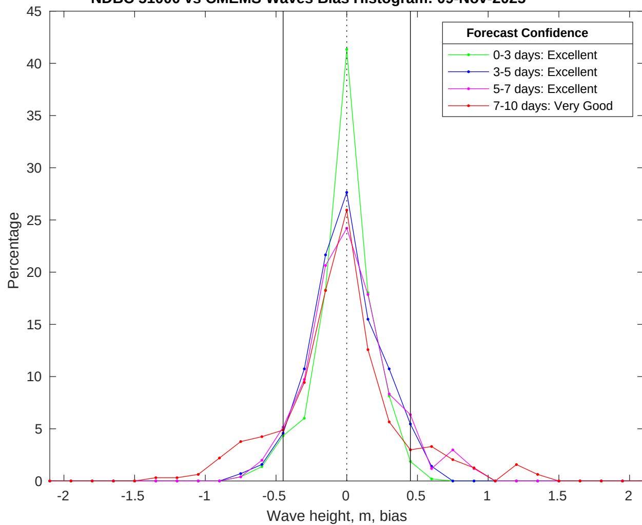
NDBC 51000 vs CMEMS Waves Bias Histogram: 09-Nov-2025
