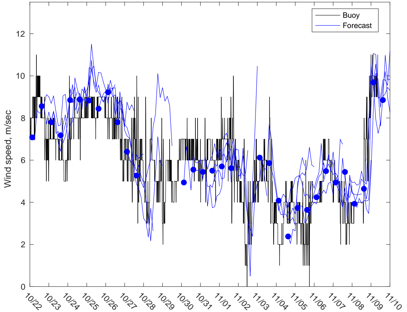
NDBC 51000 vs GFS Winds: 3 to 5 day forecast
