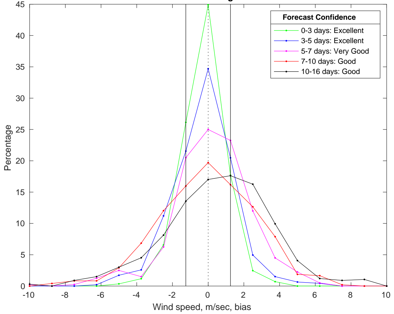
NDBC 51000 vs GFS Winds Bias Histogram: 09-Nov-2025
