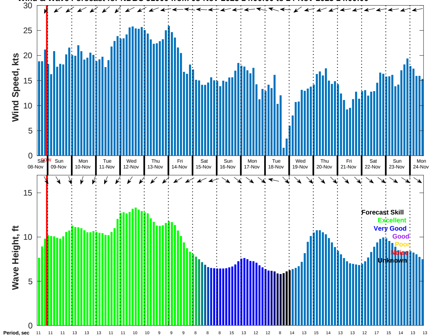
Wind & Wave Forecast for NDBC 51000 from 08-Nov-2025 14:00:00 to 24-Nov-2025 14:00:00
