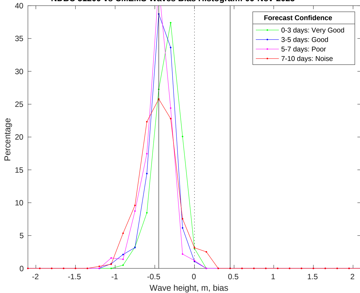
NDBC 51209 vs CMEMS Waves Bias Histogram: 09-Nov-2025
