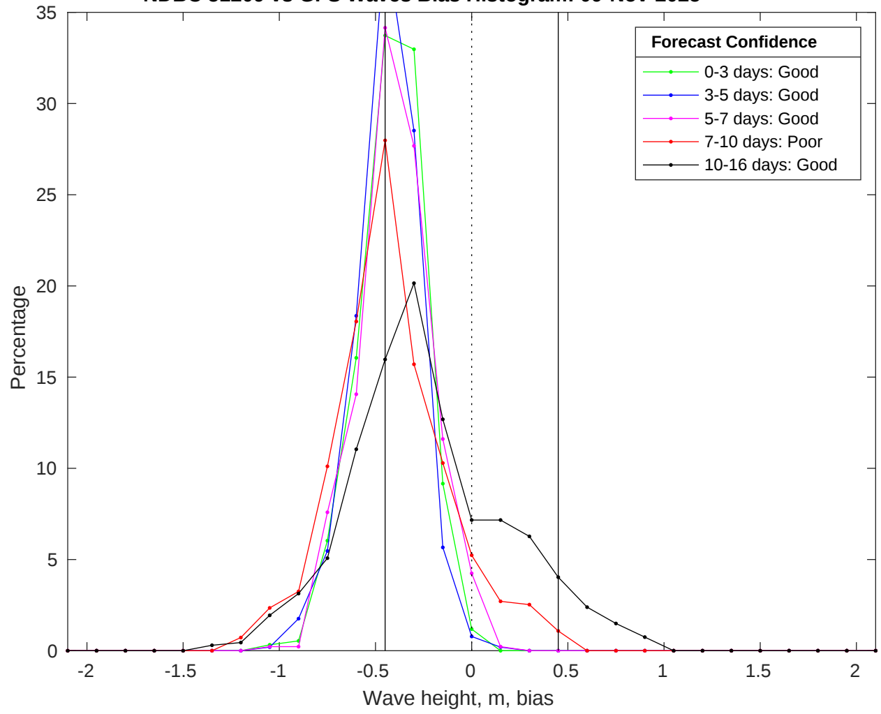
NDBC 51209 vs GFS Waves Bias Histogram: 09-Nov-2025
