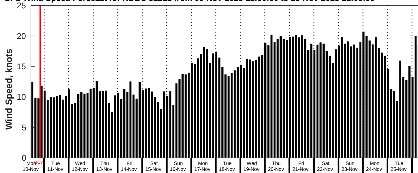
GFS Wind Speed Forecast for NDBC 52211 from 09-Nov-2025 11:00:00 to 25-Nov-2025 11:00:00
