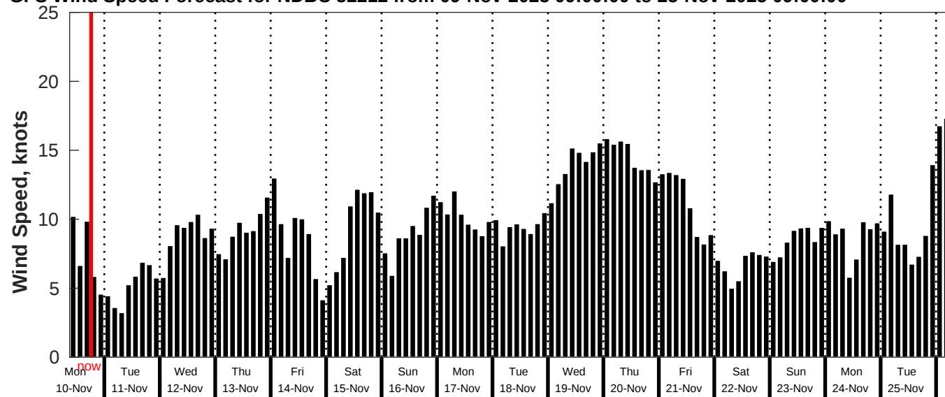
GFS Wind Speed Forecast for NDBC 52212 from 09-Nov-2025 09:00:00 to 25-Nov-2025 09:00:00
