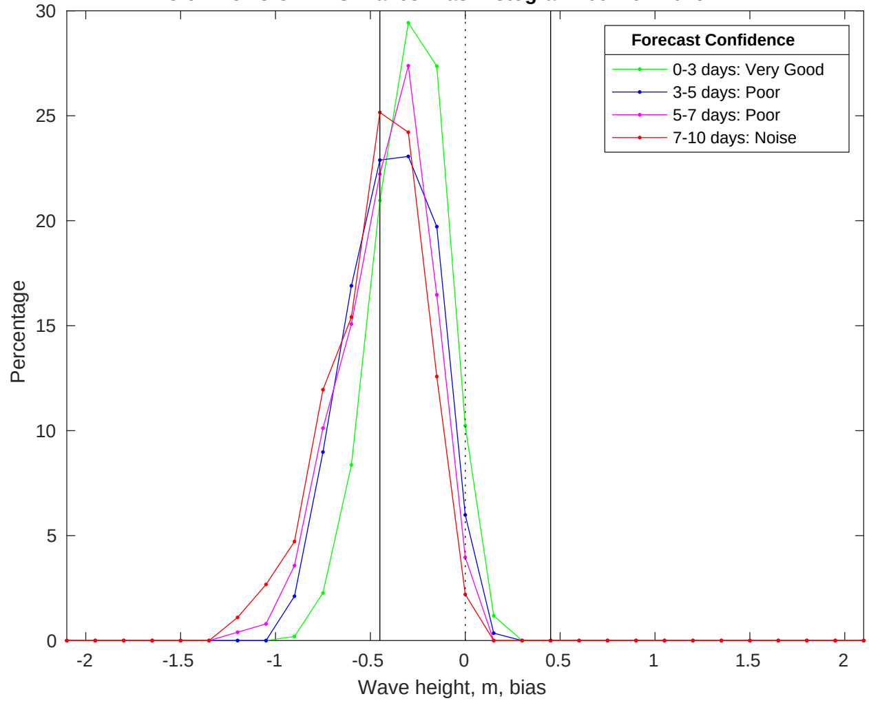
NDBC 52213 vs CMEMS Waves Bias Histogram: 09-Nov-2025
